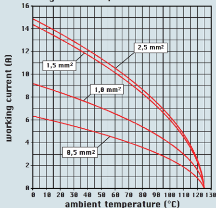
diagram CDD 24 poles
