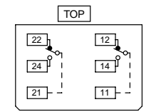
SPDT/DPDT Contacts
