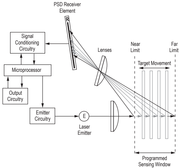
Figure 2. Using optical triangulation to determine sensing distance
