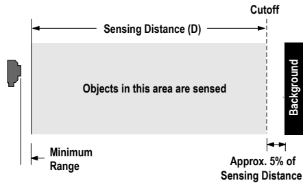
Figure 3. Background Suppression SET
